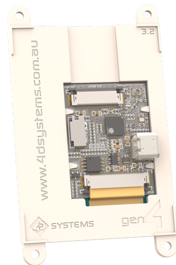
gen4-ESP32-32CT Rear
