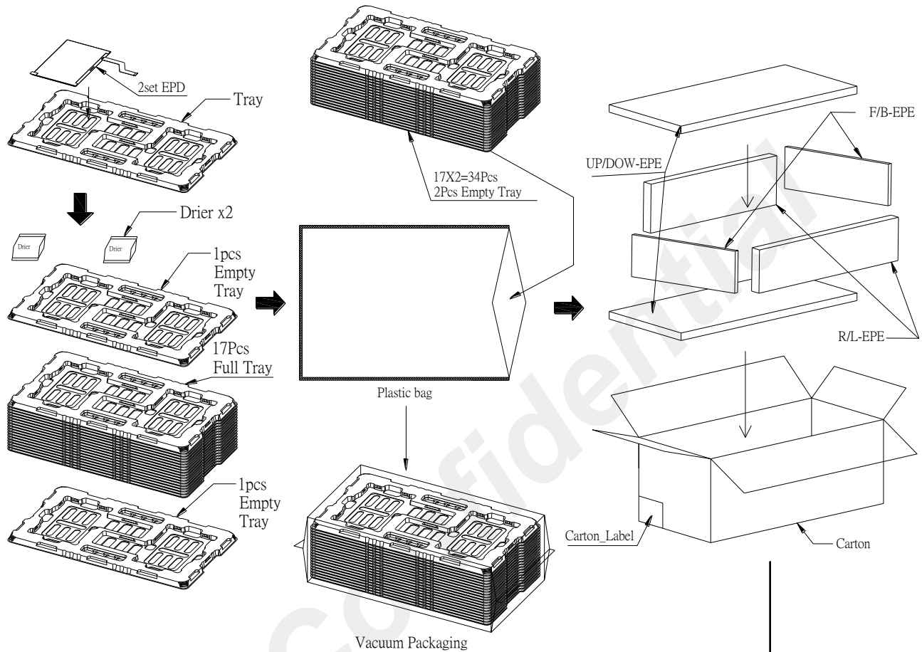
Figure 7-1 Packing Diagram
