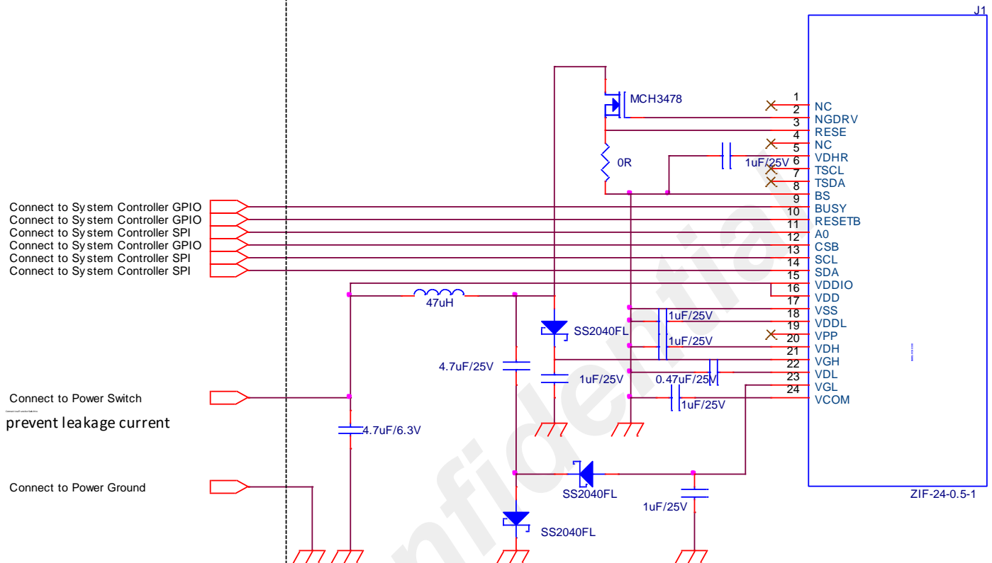
Figure 5-1 EPD Reference Circuit
