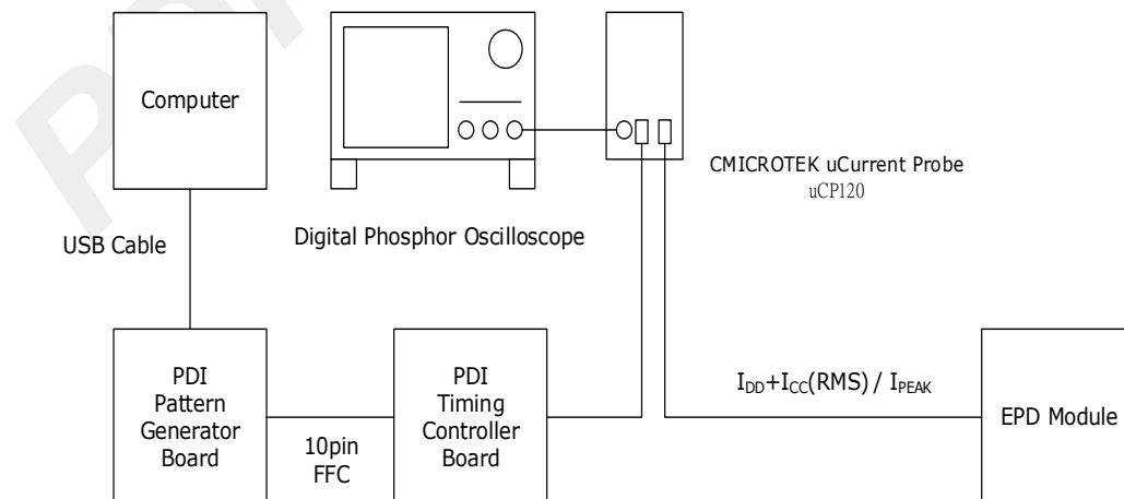
Figure 3-3 Current Measurement
