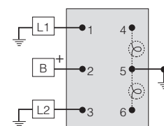
SPDT On-Off-On or On-On Independent (4 terminals)
