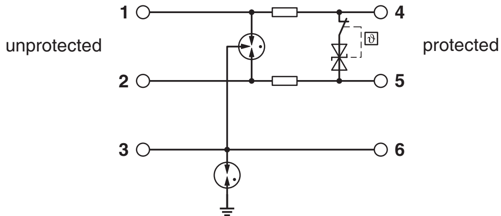
Circuit diagram
