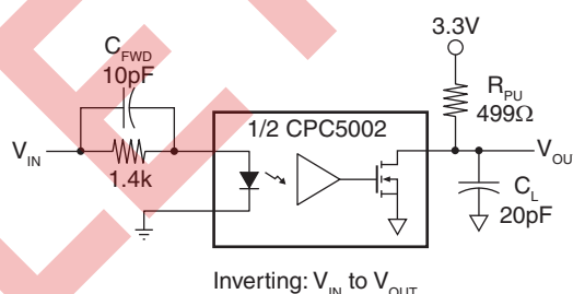
Figure 1. Inverting Configuration
