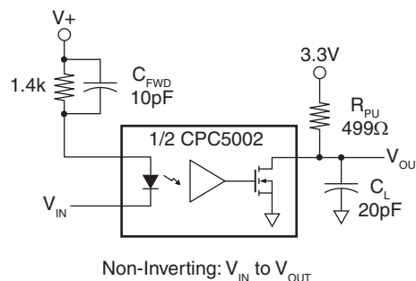
Figure 2. Non-Inverting Configuration
