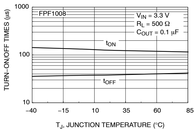
Figure 13. FPF1008 t_{ON} / t_{OFF} vs. Temperature
