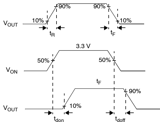
Figure 32. Timing Diagram
