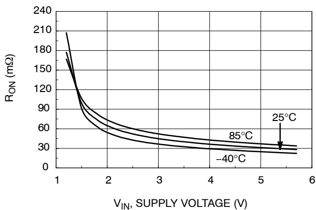
Figure 11. R_{ON} vs. V_{IN}
