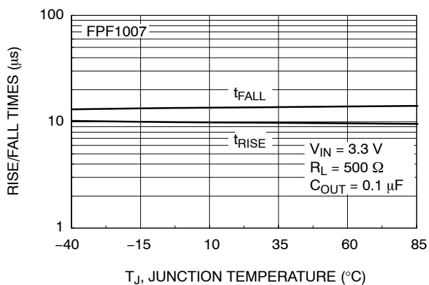
Figure 15. FPF1007 t_{RISE} / t_{FALL} vs. Temperature
