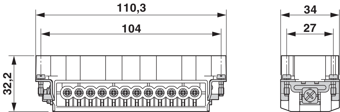
Dimensional drawing
