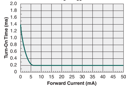
Typical Turn-On Time vs. LED Forward Current ( I_L=1\text{A}_{DC} )
