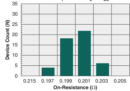
Typical On-Resistance Distribution (N=50, I_F=10\text{mA} , I_L=1\text{A}_{DC} )
