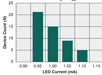
Typical I_F for Switch Dropout (N=50, I_L=1\text{A}_{DC} )
