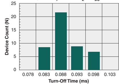
Typical Turn-Off Time (N=50, I_F=10\text{mA} , I_L=1\text{A}_{DC} )
