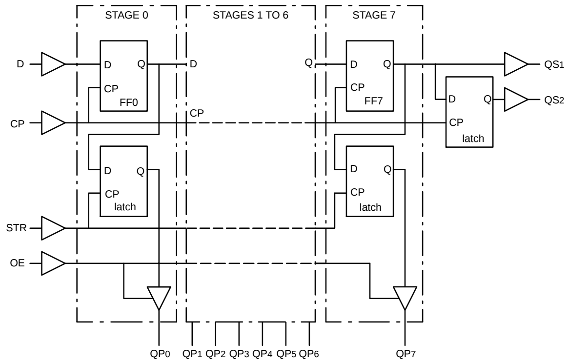
Figure 5. Logic Diagram
