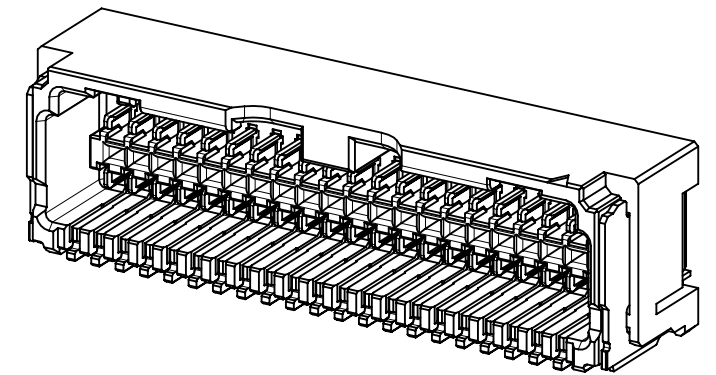
42極 42 CIRCUIT
