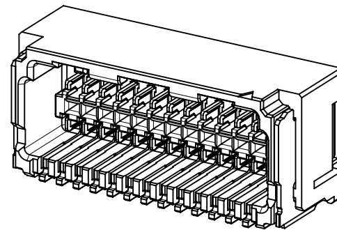
26-32極 26-32 CIRCUIT
