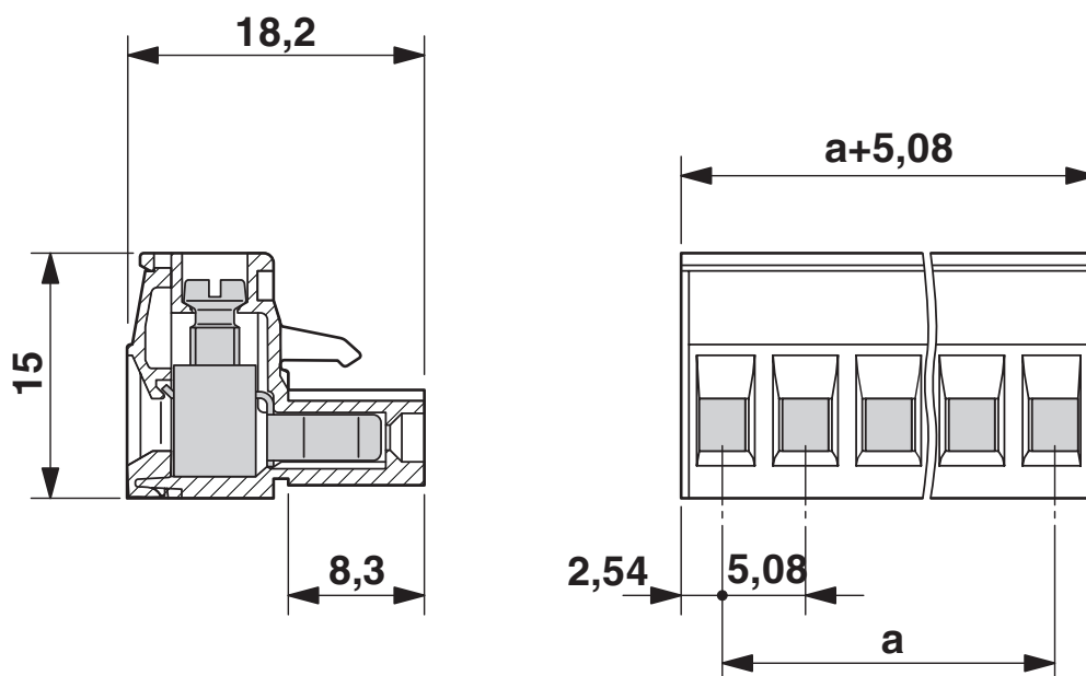
Dimensional drawing
