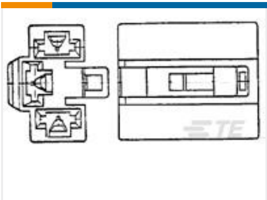
TE Part # 176774-1 FF 250 PLUG HSG 3P NYLON NAT
