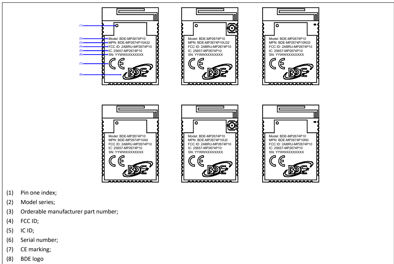
Figure 5. Module Marking
