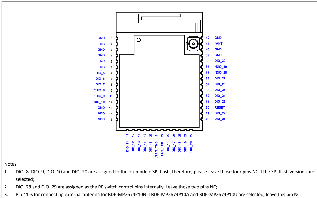
Figure 2. Pin Diagram of BDE-MP2674P10A (Top View)
