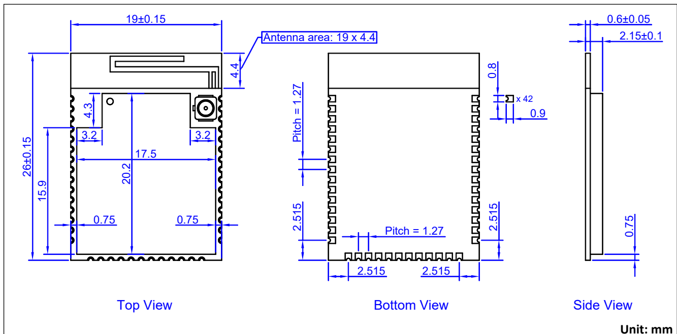
Figure 3. Mechanical Drawing of BDE-MP2674P10
