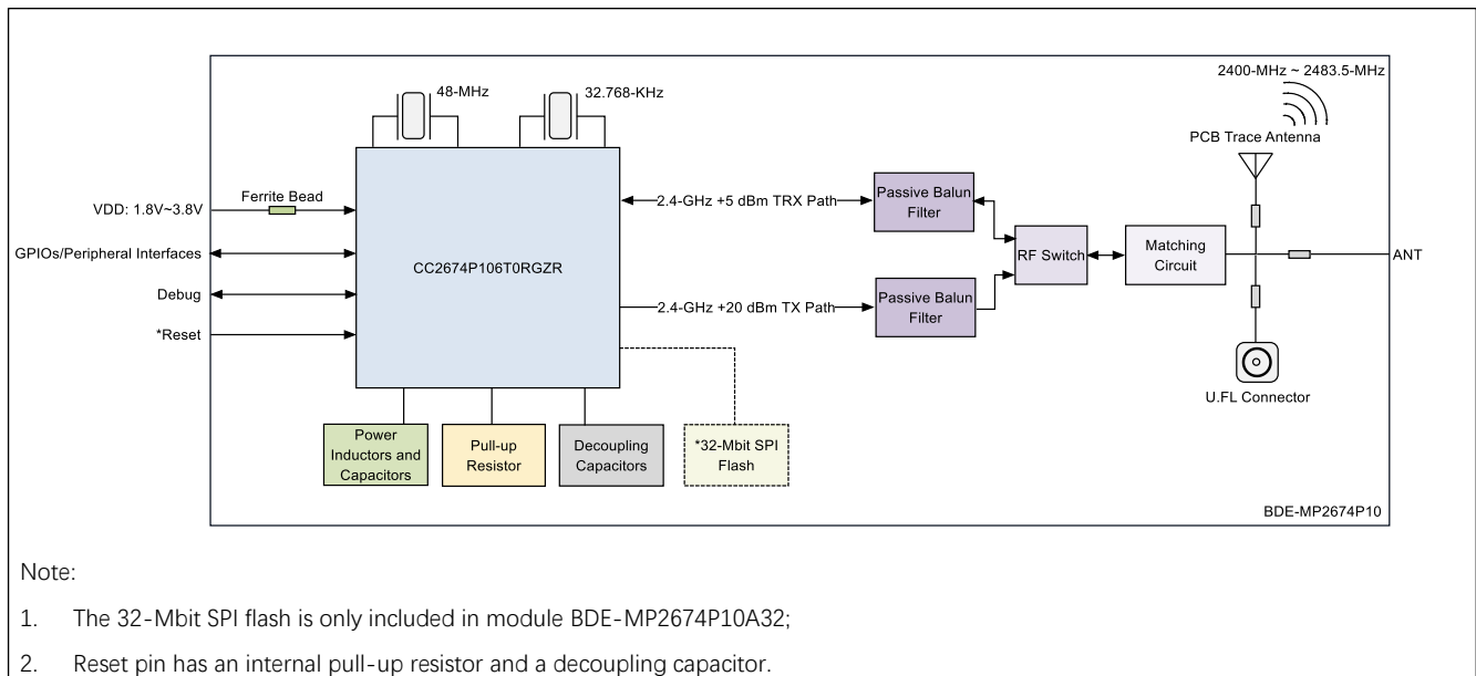
Figure 1. BDE-MP2674P10 Module Block Diagram
