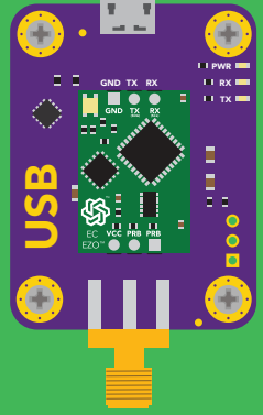
USB carrier board
