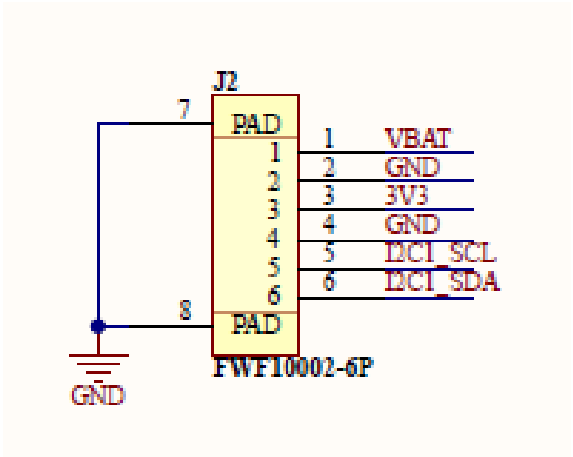
Figure 10: J2 Connector Pinout
