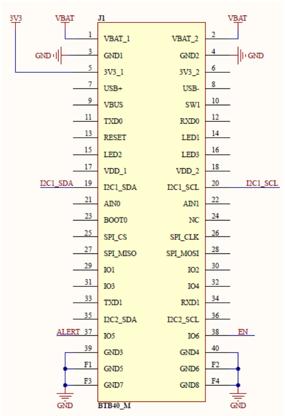
Figure 11: RAK12009 Module 40-pin WisConnector
