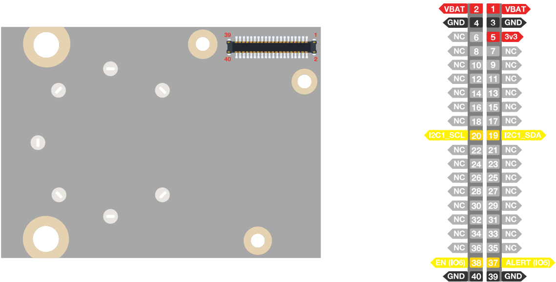
Figure 2: RAK12009 WisBlock MQ3 Alcohol Sensor Pinout
