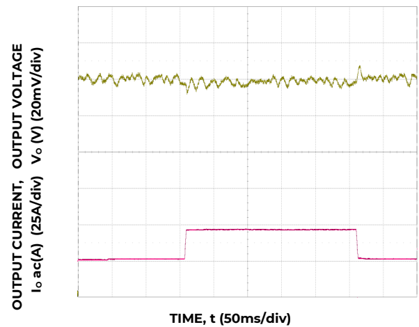
Figure 10. Trans. Resp. to 10A/ \mu\text{s} Load Change from 25% to 75% at 12V IN , C_o = 4 \times 0.047\mu\text{F} + 4 \times 0.1\mu\text{F} + 15 \times 22\mu\text{F} + 73 \times 47\mu\text{F} + 6 \times 470\mu\text{F} polymer
