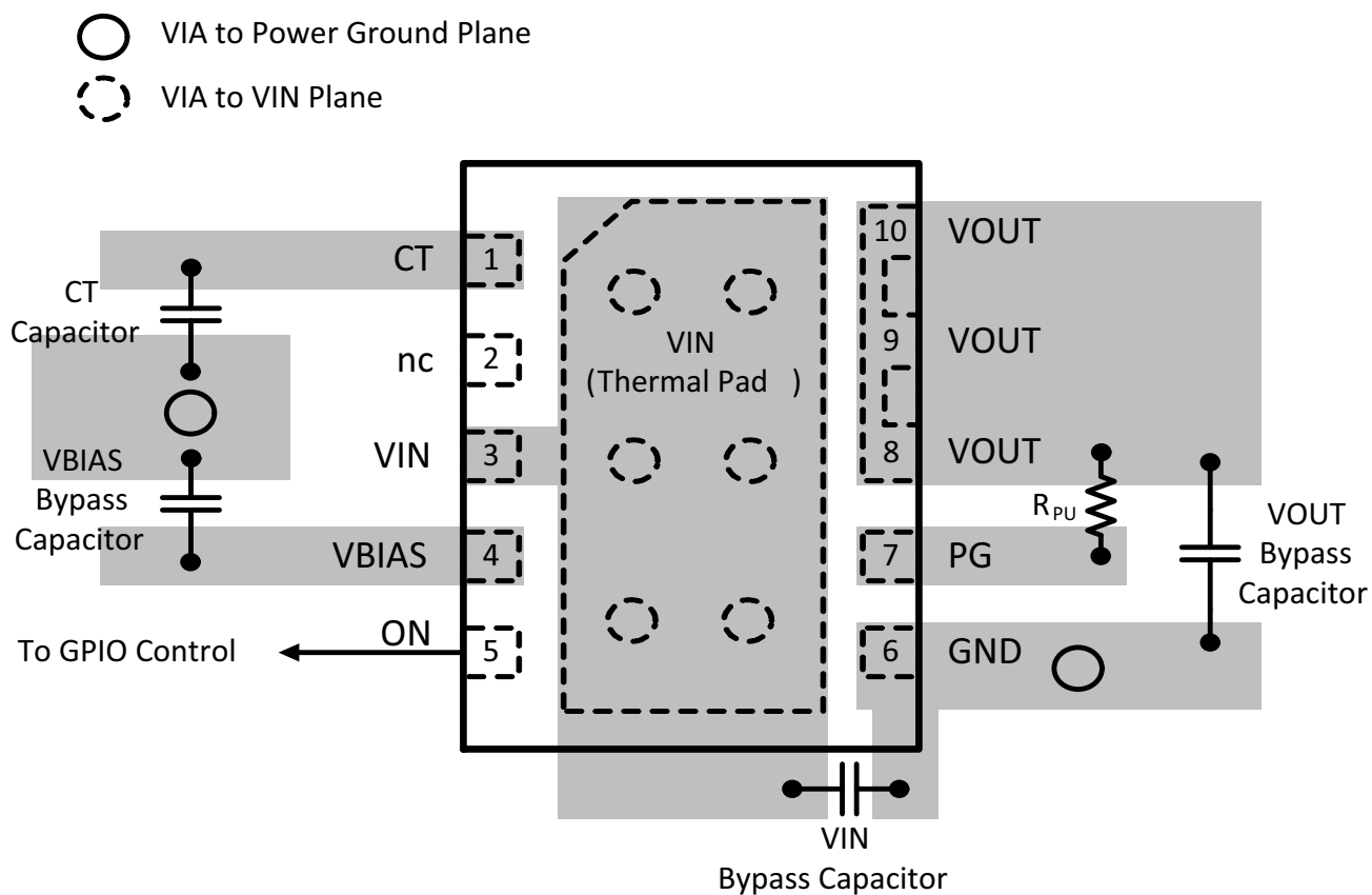
Figure 43. Layout Example
