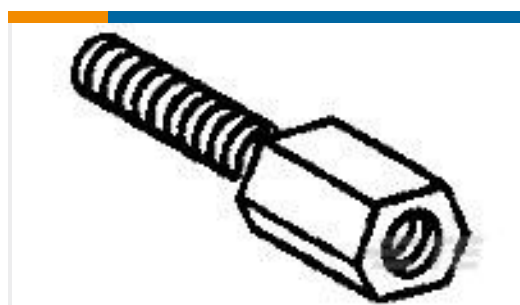
TE Part # 5747404-3 FEMALE SCRLOCK, METRIC, ZN PLTD
