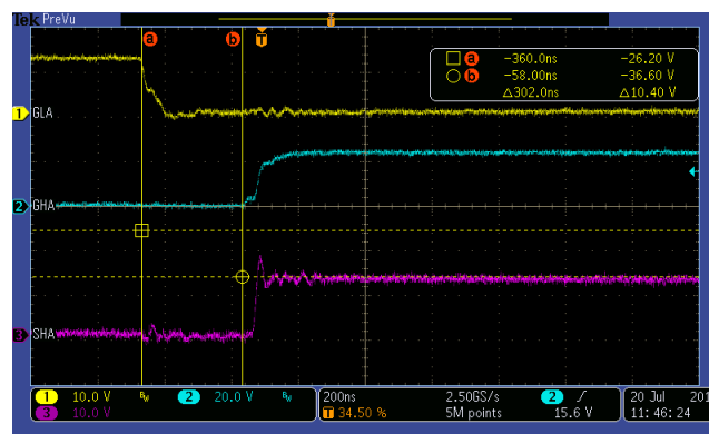
Figure 2: Dead Time
