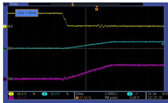
Figure 6: Switching with 100\Omega Resistance and Diode
