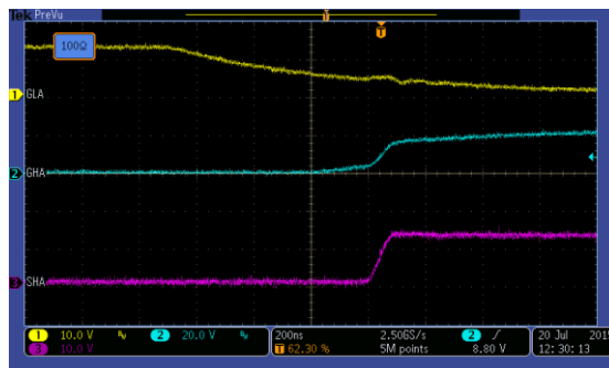
Figure 5: Switching with 100\Omega Series Resistance
