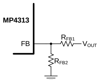
Figure 6: Feedback Network
