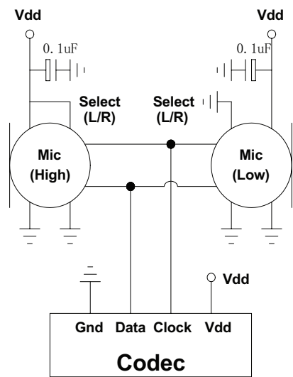
Dual Microphone
