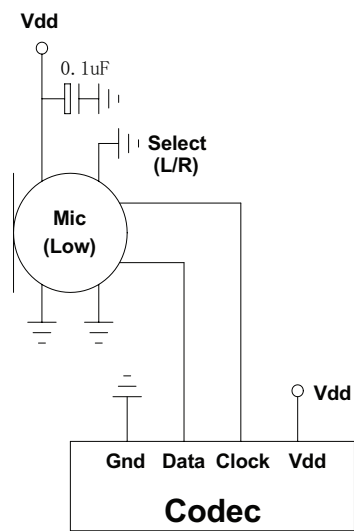
Single Microphone
