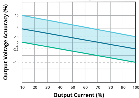
OUTPUT REGULATION CURVE 3.3, 5 Vdc input model / 5, 9, 12, 15, 24 Vdc output models (nominal input)
