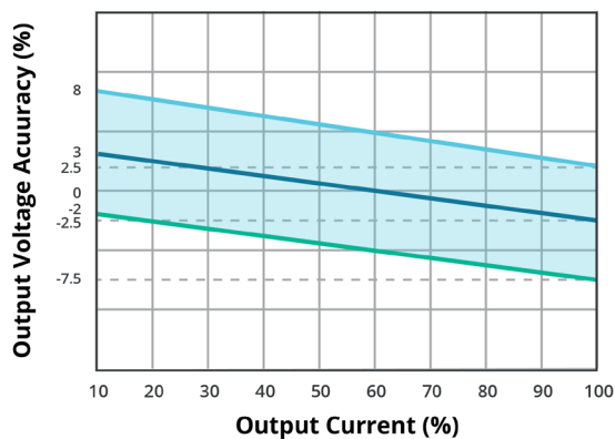
OUTPUT REGULATION CURVE all other input models / 5, 9, 12, 15, 24 Vdc output models (nominal input)
