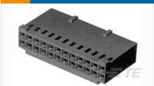
TE Part # 280513 AMPMODU II REC. HSG, DUAL ROW, 18 POS
