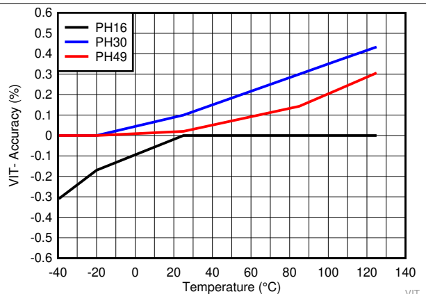
Figure 12. Negative-going Input Threshold Accuracy over Temperature for TPS3840PH-Q1
