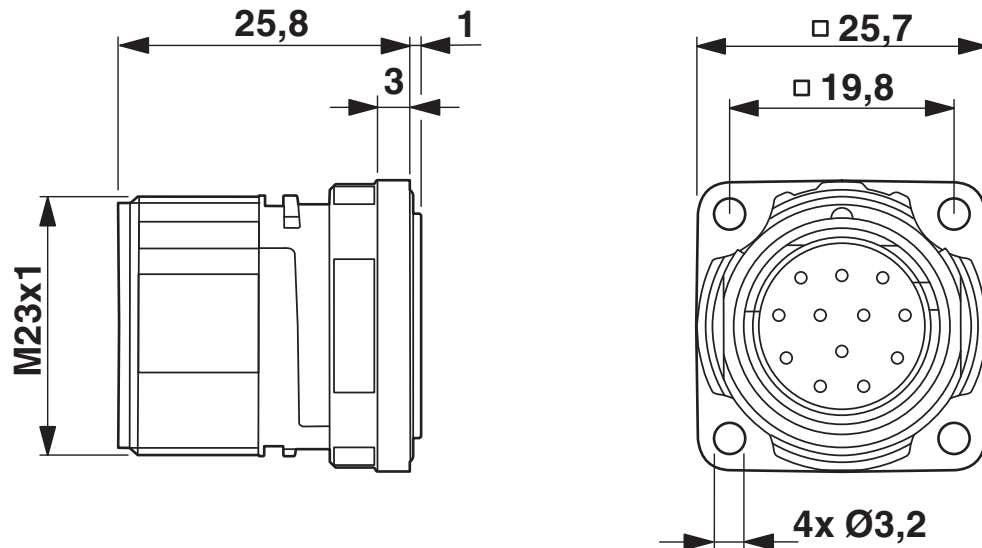
Dimensional drawing
