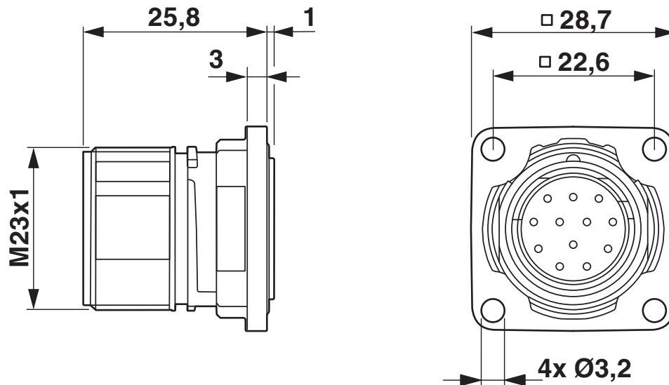
Dimensional drawing
