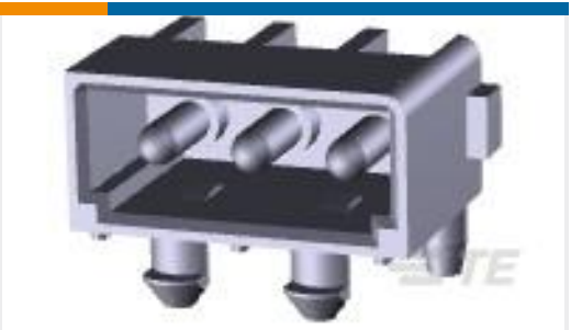
TE Part # 643488-1 03P CMNL HDR ASSY R/A
