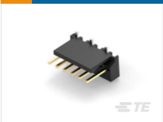
TE Part # 3-647502-6 PCB Header: Nylon, Vertical, Surface Mount, MTA 100
