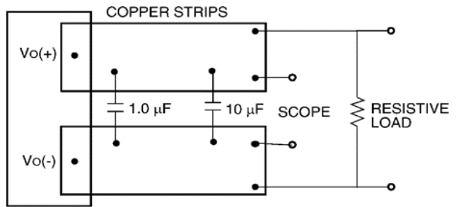
Figure 12. Output Ripple and Noise Test Setup.
