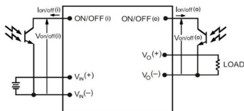
Figure 14. Remote On/Off Implementation.
