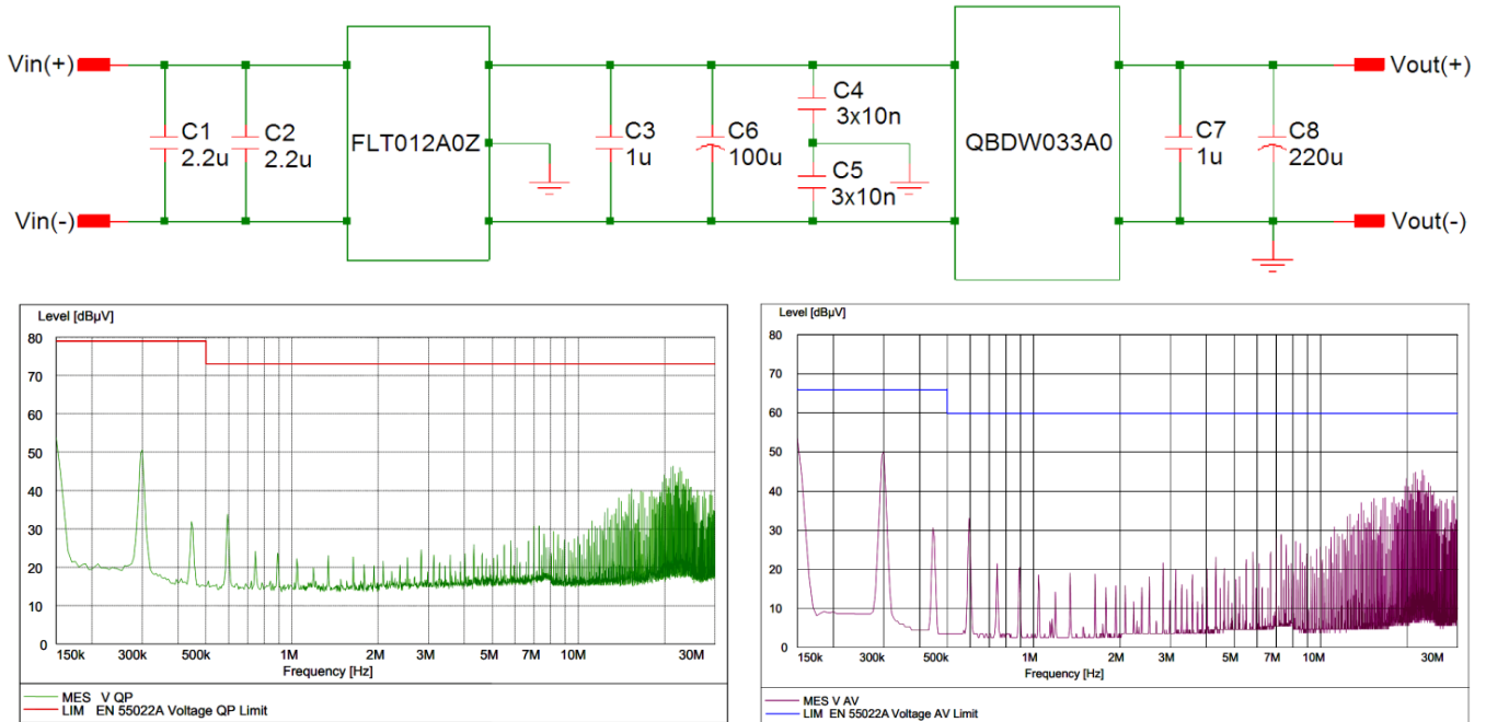
Figure 25. EMC Consideration
