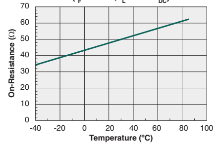
Typical On-Resistance vs. Temperature ( I_F=10\text{mA} , I_L=50\text{mA}_{DC} )
