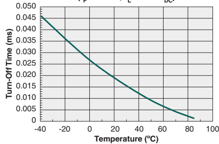
Typical Turn-Off Time vs. Temperature ( I_F=10\text{mA} , I_L=50\text{mA}_{DC} )
