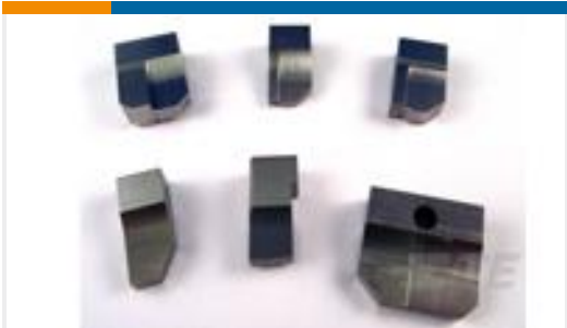
TE Part # 852141-1 ANVIL, LEFT (DUAL)
