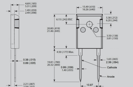
TO-247 2-Lead
