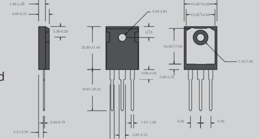
TO-247-3-Lead
