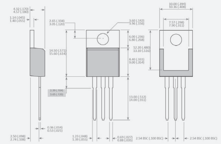
TO-220 3-Lead
