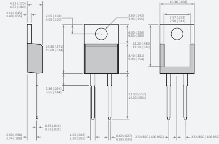
TO-220 2-Lead
