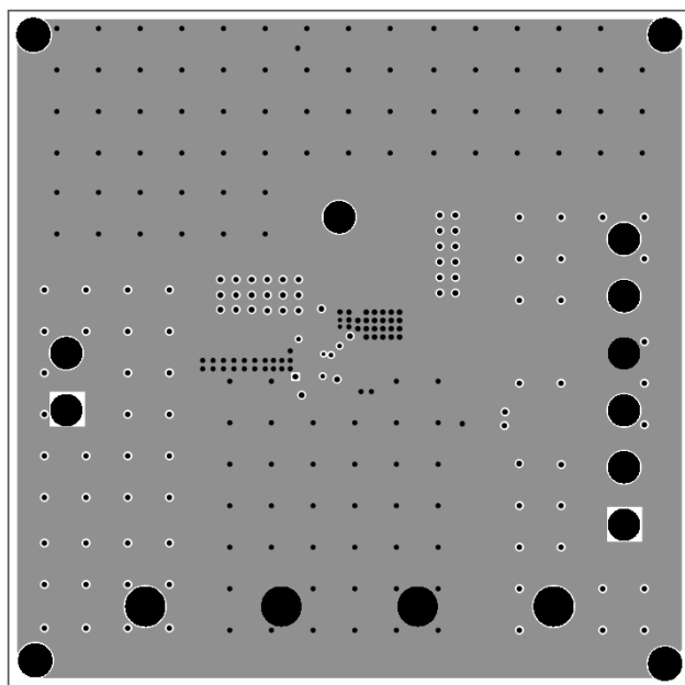
Figure 3: Inner Layer1
