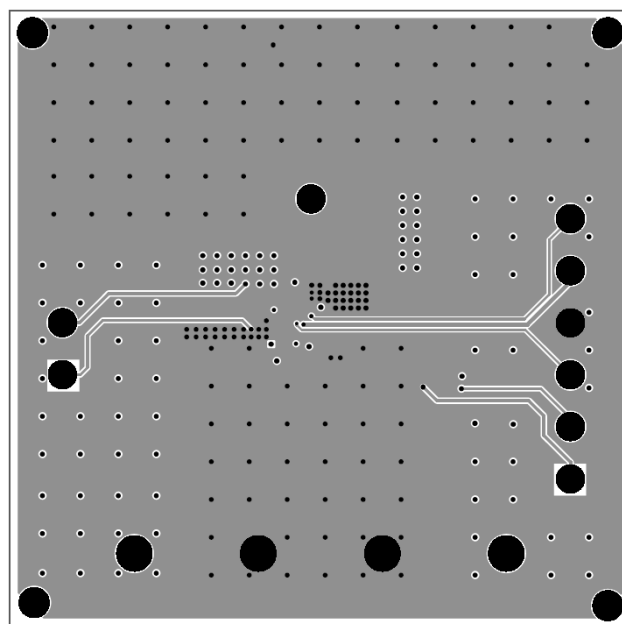
Figure 4: Inner Layer2
