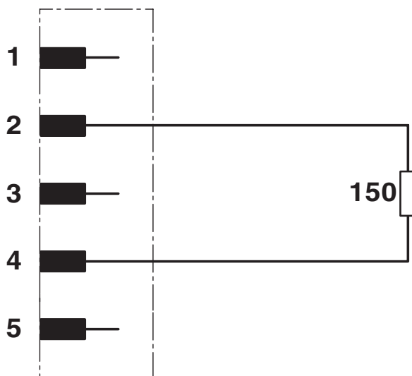
Circuit diagram
