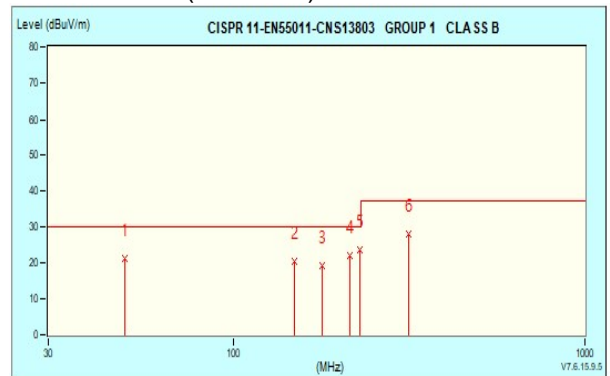
EMI: FCC "B" (Radiation)
