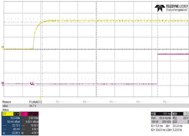
PG(Input voltage: 85Vac) rated load
