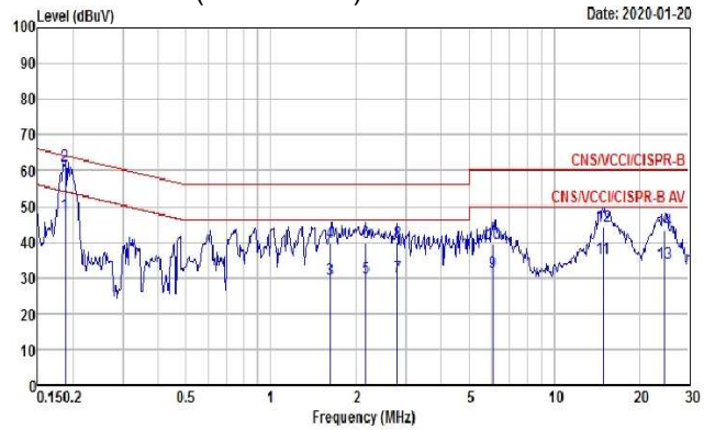
EMI: FCC "B" (Conduction)
