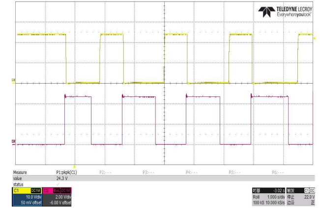
Remote on off
