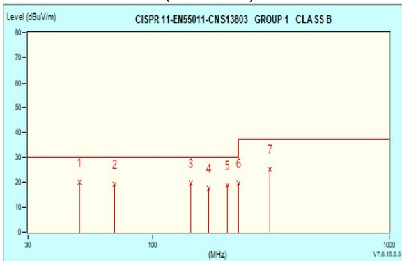
EMI: EN55011 "B" (Radiation)
