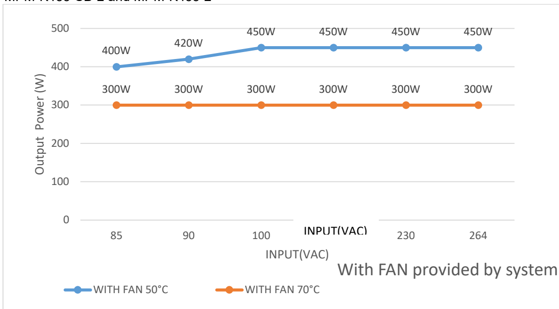
MPM-K455-SB-1 and MPM-K455-1 (Fan provided by customer) MPM-K455-SB-2 and MPM-K455-2
