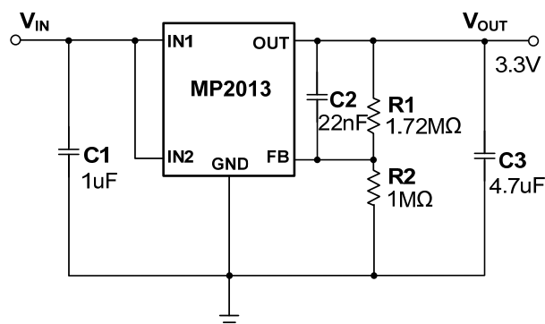
Figure 6: Design Example
