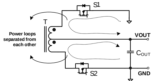
Figure 9: System Power Loop
