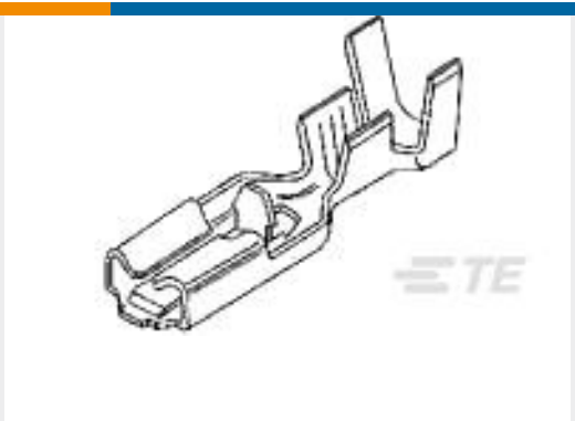
TE Part # 63239-1 POSITIVE LOCK 250 REC 12-10 AWG TPBR
