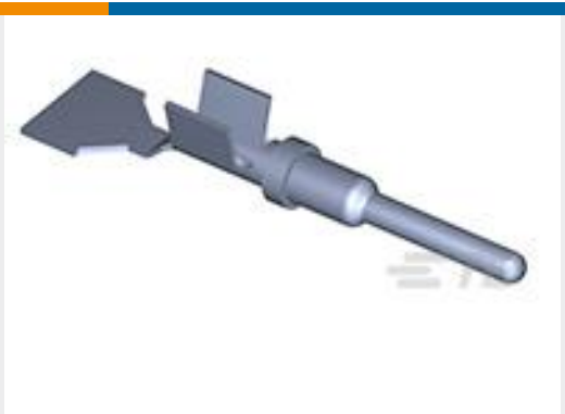
TE Part # 638112-1 PIN, SF, SIZE 16, 14-18 AWG,NO INS, AU/SN
