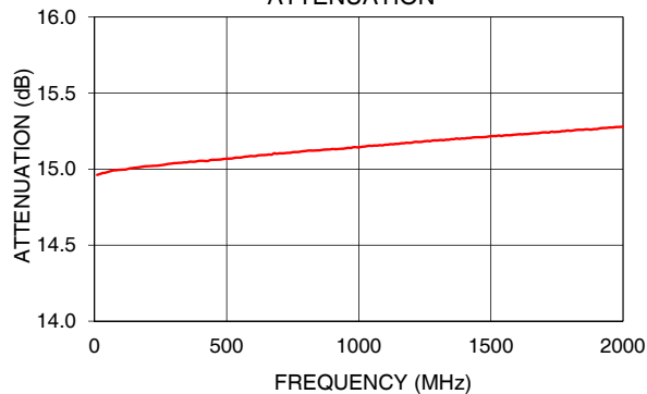
HAT-15A+ ATTENUATION
