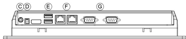
Bottom View
