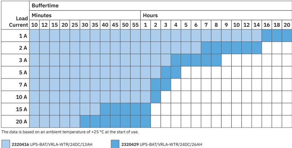
Buffer times for TRIO DC UPS for VRLA-WTR battery modules
