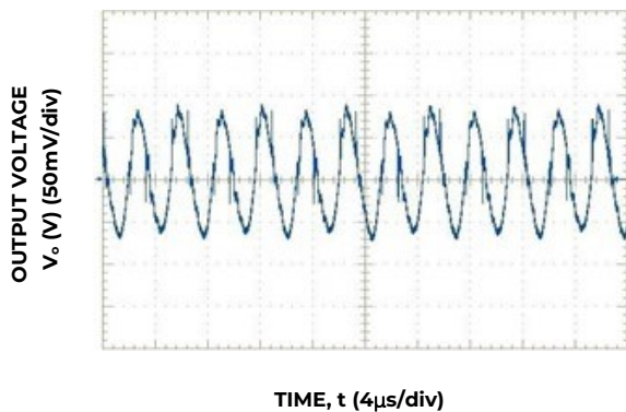
Figure 2. Typical output ripple and Noise at Room Temperature and 48\text{V}_{in} ; I_o = I_{o,max} ; C_{o,ext} = 440\mu\text{F} .
