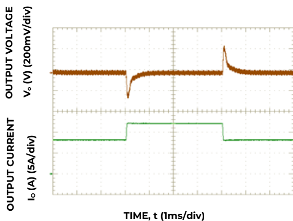
Figure 3. Dynamic Load Change Transient Response from 50% to 75% to 50% of Full Load at Room Temperature and 48\text{V}_{in} ; 0.1\text{A}/\mu\text{s} , C_{o,ext} = 470\mu\text{F} .
