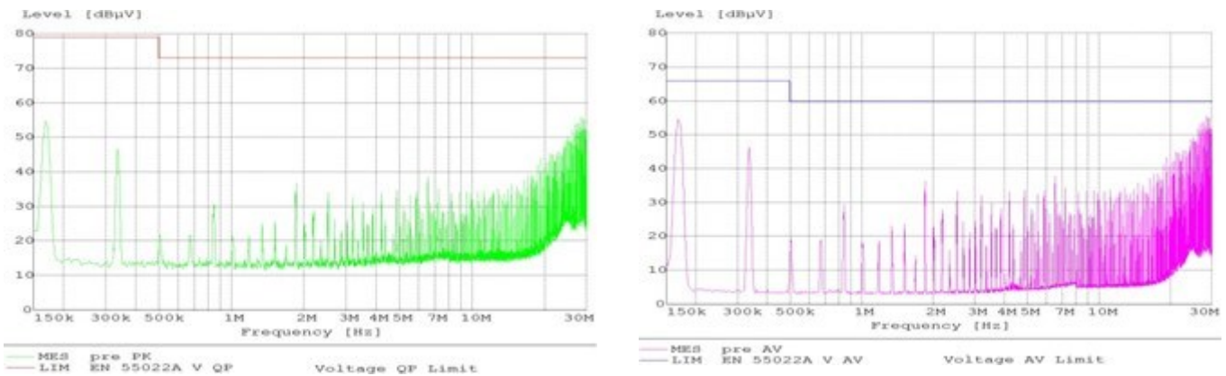
Figure 23. EMC Filter
