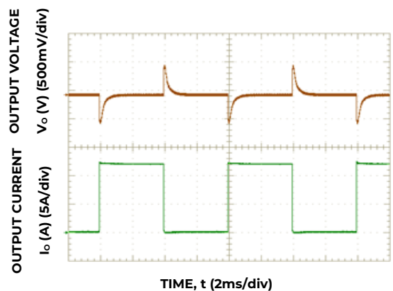
Figure 6. Dynamic Load Change Transient Response from 0% to 75% to 0% of Full Load at Room Temperature and 48\text{V}_{in} ; 2.0\text{A}/\mu\text{s} , C_{o,ext} = 880\mu\text{F} .
