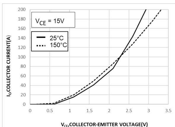
Figure 5. Typical Saturation Voltage Characteristics
