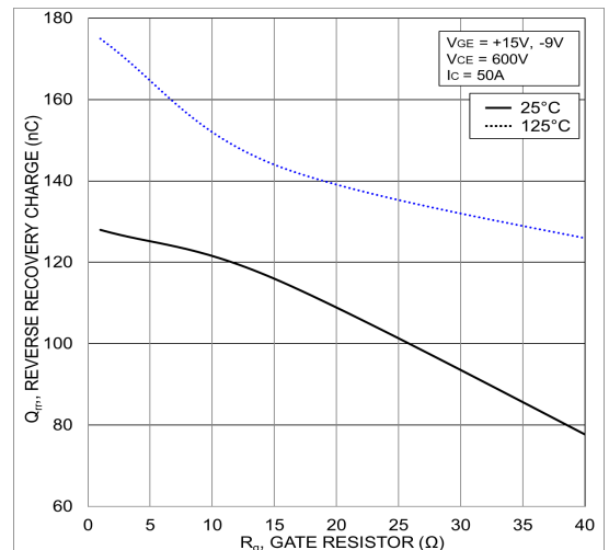
Figure 19. Typical Reverse Recovery Charge vs. R_g
