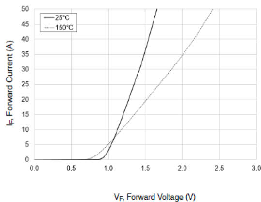
Figure 7. Boost Diode Forward Characteristics
