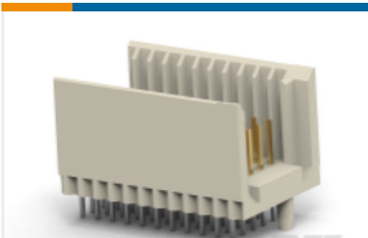
TE Part # 5188835-1 Hard Metric Male Connector: Traditional Backplane, Mezzanine, 2mm
