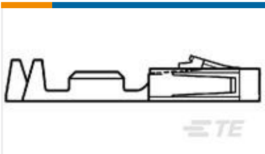
TE Part # 104481-8 SHORT POINT RECPT CONT LP
