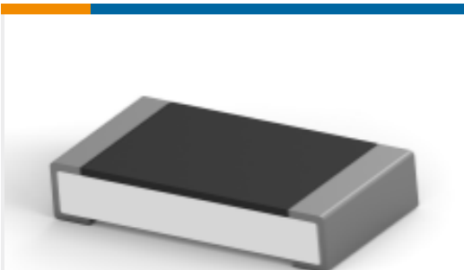
TE Part # 3-2176388-9 RQ 1206 24R9 0.1% 10PPM 5K RL
