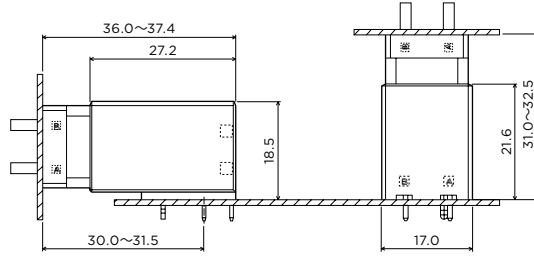
Horizontal /Vertical type
