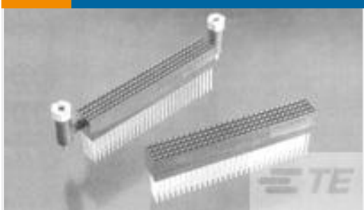
TE Part # 1375799-2 ASSY, 120 POS PC104 PLUS
