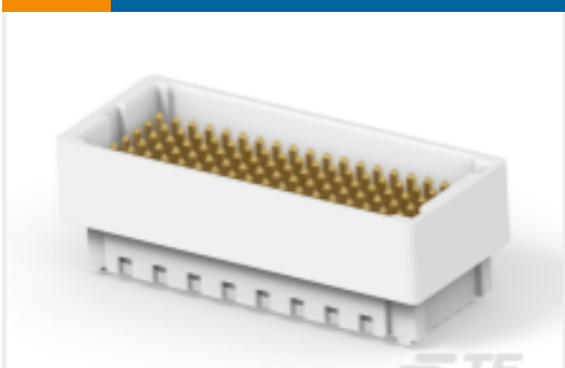
TE Part # 2102060-2 High-speed Mezzanine Connector: Pin & Socket Connector
