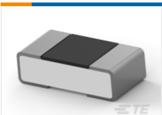
TE Part # 3-2176364-5 RQ 0402 10K5 0.1% 10PPM 5K RL
