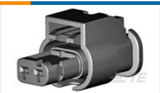
TE Part # 1-1670916-1 2POS, MCON 1.2 LL REC SEALED
