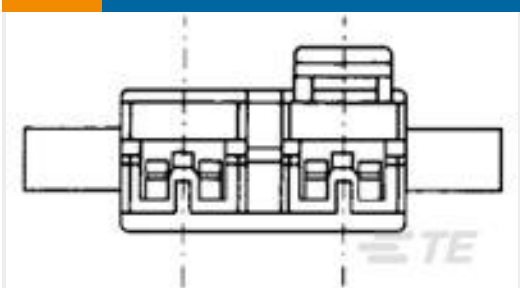
TE Part # 353253-1 PL EX 110 (2.8 MM) HOUSING RECEPTACLE
